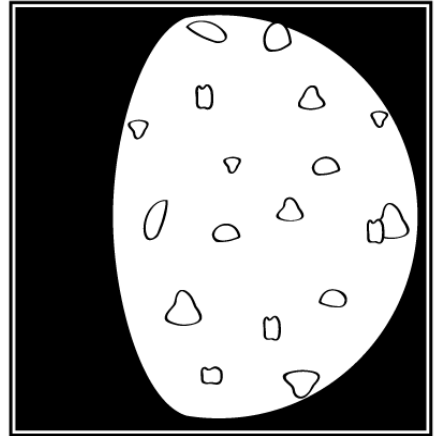
WAXING GIBBOUS
