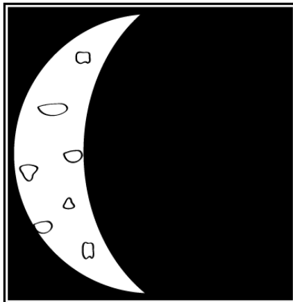
WANING CRESCENT
