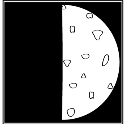
FIRST QUARTER
