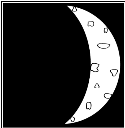
WAXING CRESCENT
