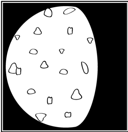
WANING GIBBOUS
