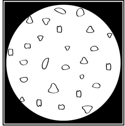
FULL MOON
