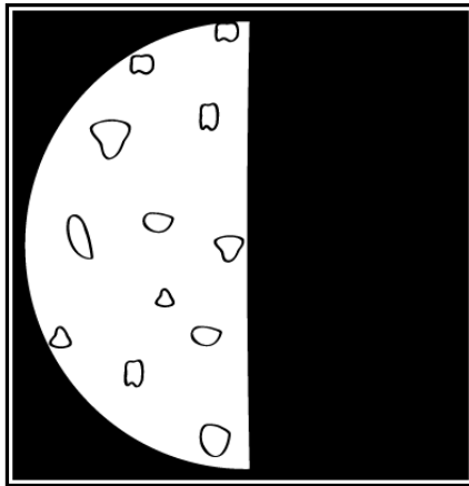
LAST QUARTER
